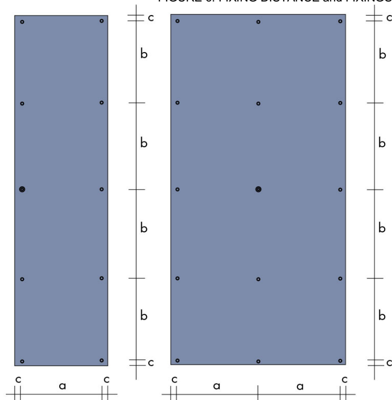
FIGURE 6: FIXING DISTANCE and FIXINGS HOLES DIMENSIONS
