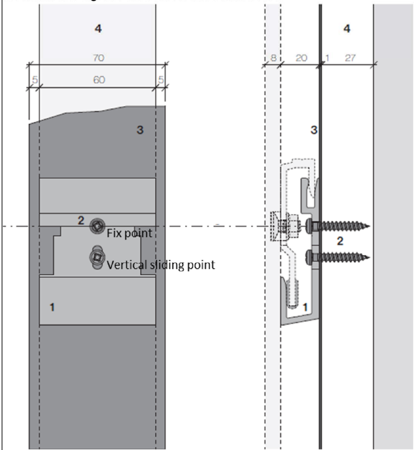
Installation U-agraffe on vertical subconstruction
